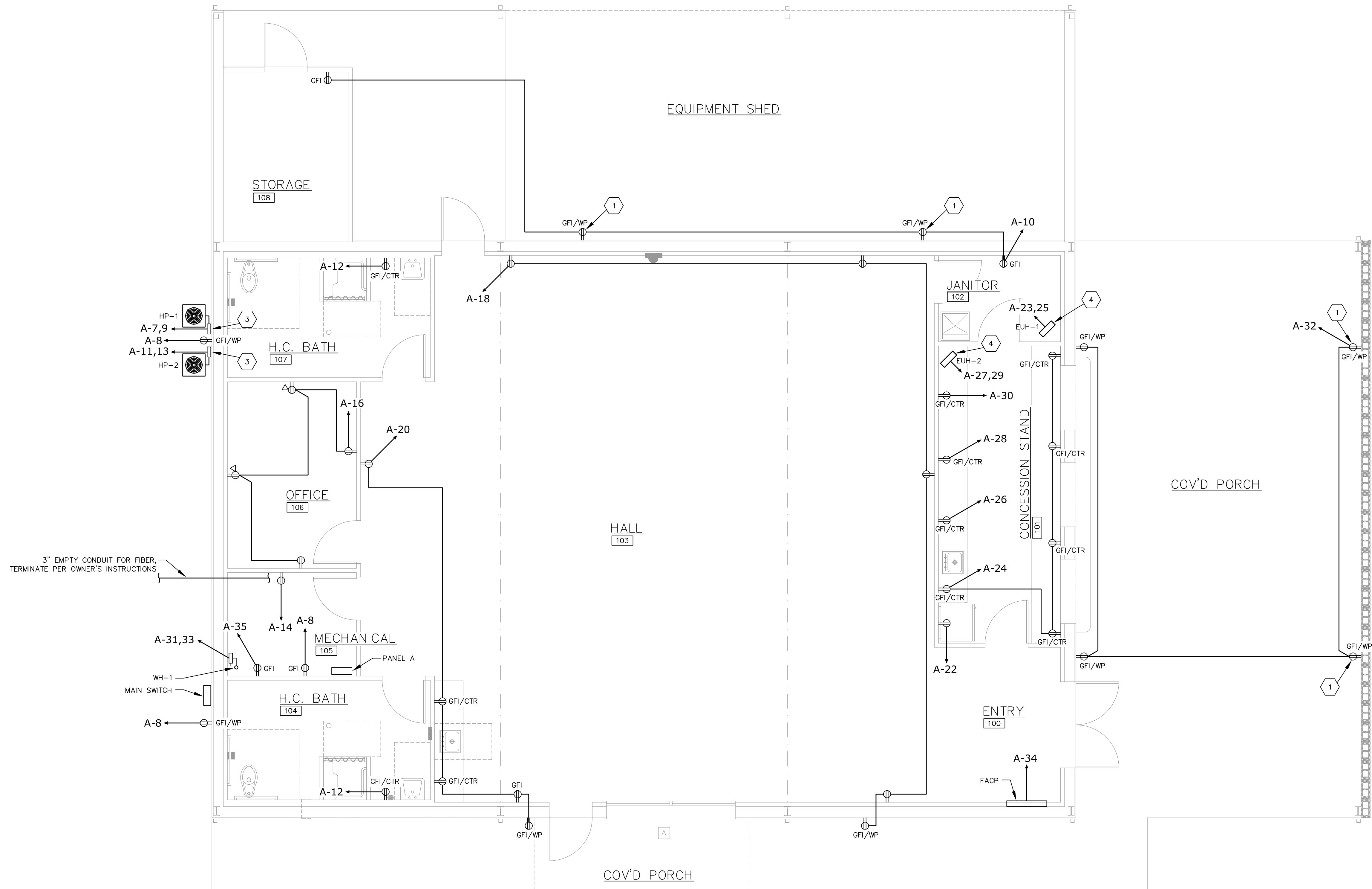
FLOOR PLAN - POWER SCALE: 1/4"=1'-0"
